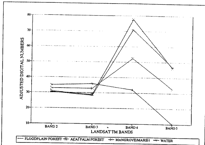
Figure 3. Spectral curves of Floodplain Forest, Açai palm forest, and associated features using Landsat TM data from July, 1991, Marajó Island, Brazil.
